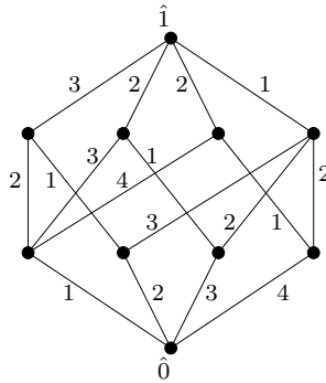
FIGURE 1. An EL-labeling of the rank 3 near pencil on 4 atoms.
