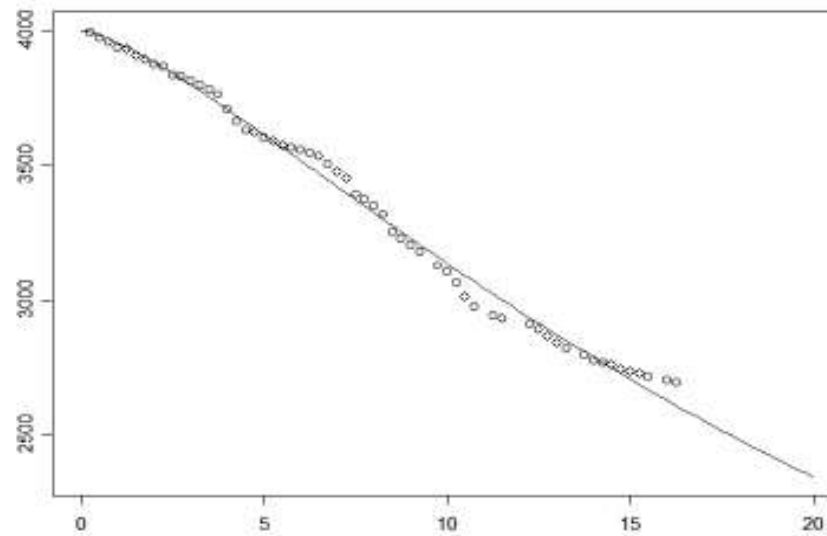
Matis and Hartley 1971 sheep 148 data and LL2 fit
