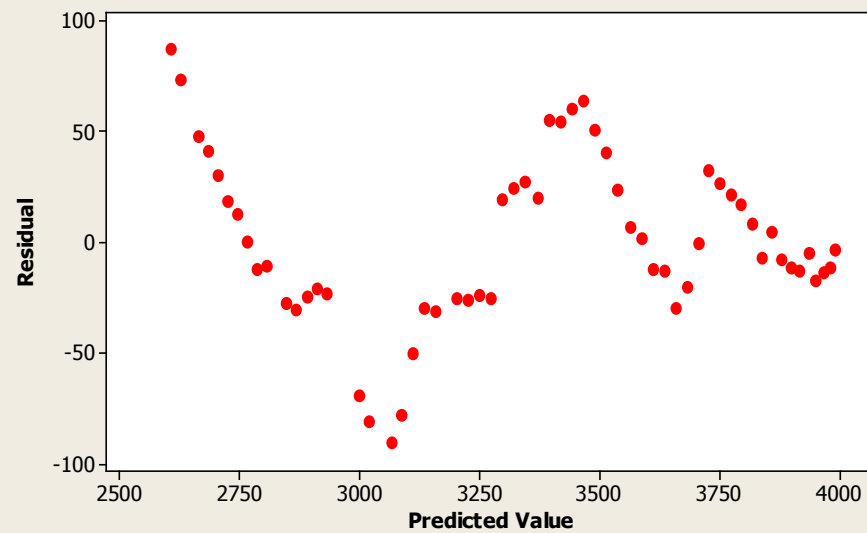
Scatterplot of Residual vs Predicted Value
