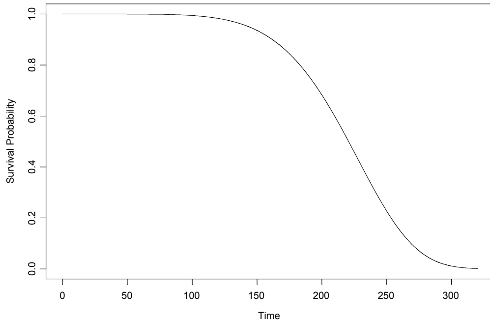
Estimated Survival Function: Weibull2 Fit
